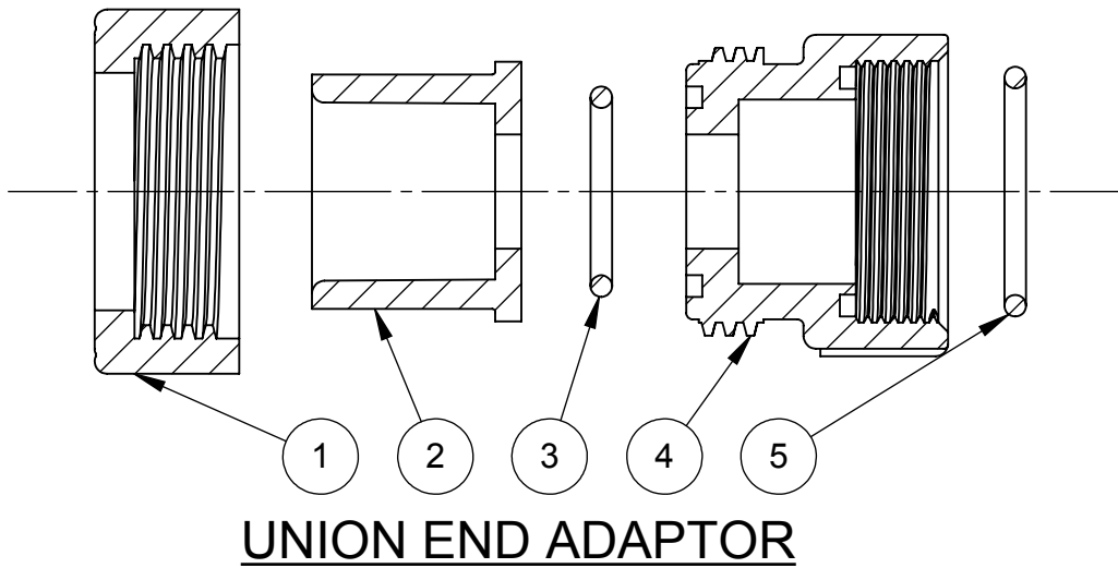
SERIES 520 UNION END ADAPTOR KITS
