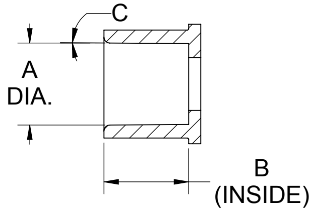
FEMALE SOCKET WELD END CONNECTOR
